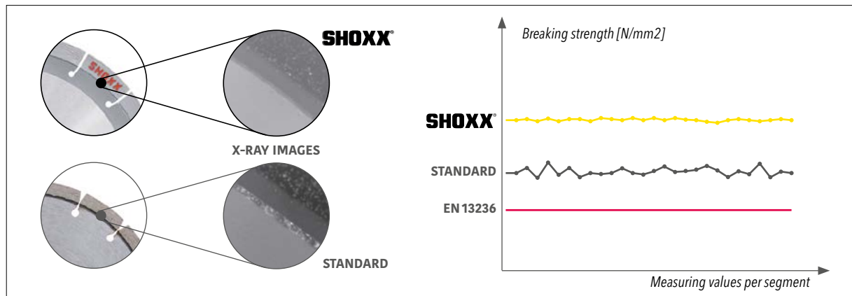
Deep and porefree welding of the SHOXX segments
